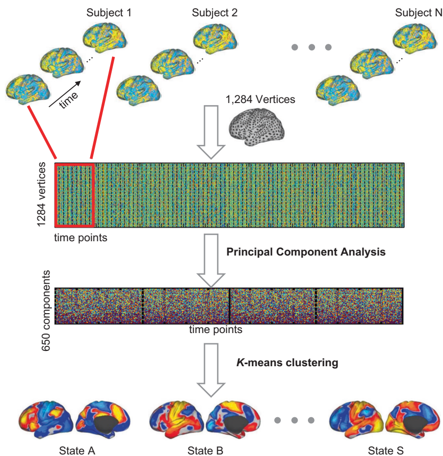
Fig. 1 Strategy for estimating brain network states from resting state fMRI. BOLD images were clustered into brain states according to their spatial patterns, i.e., images with similar spatial patterns were clustered together. Specifically, the preprocessed fMRI data of each individual subject was projected to the FreeSurfer fsaverage3 surface space, which consisted of 1284 vertices in total. The data of different time points of each subject were aligned to construct a spatiotemporal matrix (indicated by the red rectangle). The data of all subjects were
