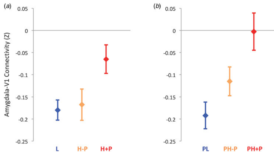
Fig. 3. Amygdala-V1 connectivity is elevated in individuals with, compared to those without, persecutory beliefs. In an ROI analysis, average amygdala-V1 connectivity values ( z scores) were extracted. The mean values are plotted here for the following groups: members of the H group with persecutory beliefs (H + P, n = 19 ), the H group without persecutory beliefs (H - P, n = 24 ), and the L group (L, n = 43 ) in (a); and members of the PH group with persecutory beliefs (PH + P, n = 10 ), the PH group without persecutory beliefs (PH - P, n = 12 ), and the PL group (PL, n = 17 ) in (b). In (a), post-hoc t tests showed that amygdala-V1 connectivity of the H + P group was significantly greater in magnitude than that of both the H - P and L groups ( p = 0.043 and p = 0.006 , respectively), while there was no significant difference between the H - P and L groups ( p = 0.760 ) in amygdala-V1 connectivity. Similarly, the PH + P group showed significantly greater amygdala-V1 connectivity compared to both the PH - P and PL groups ( p = 0.045 and p = 0.001 , respectively), while the difference between the PH - P and PL groups did not reach significance ( p = 0.099 ). Note that the majority of the extracted z -scores are negative in value because of the effects of the global mean regression (see online Supplementary Fig. S3). Error bars represent standard errors of the mean.
