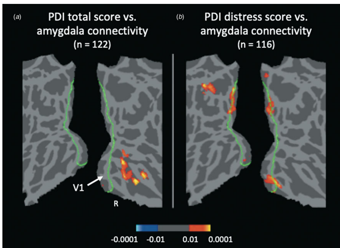
Fig. 2. The number of delusional beliefs and degree of associated distress correlate with amygdala-visual cortex connectivity. Flattened voxel-wise maps of parietal and occipital cortex showing clusters that met FDR whole-brain correction following whole-brain regression of amygdala connectivity with PDI total score (a) or PDI distress score (b) as regressors. These maps reveal similar patterns of correlations between these measures and amygdala-visual cortex connectivity [in (a), MNI coordinates of peak in temporal occipital fusiform cortex ( x, y, z ) = 36, -50, -10, z = 3.84 , p = 0.001 , 681 voxels; in (b), MNI coordinates of peak in extrastriate cortex ( x, y, z ) = 10, -54, 2, z = 3.60 , p < 0.001 , 795 voxels]. The border of V1 is shown in green. The p -values of the clusters are represented by warm (positive correlations) and cool (negative correlations) colors. Two clusters (negative correlations) in (b) are not shown; see Table 2d for details.
