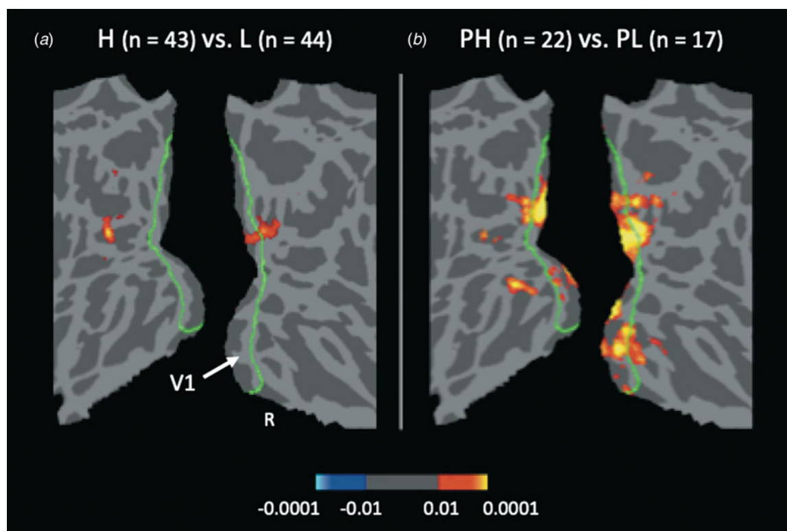
Fig. 1. Amygdala-visual cortex connectivity is elevated in youth with high levels of delusional beliefs. Flattened voxel-wise maps of parietal and occipital cortex showing clusters that met FDR whole-brain correction in the comparisons of amygdala connectivity of the H v. L groups (a); and PH v. PL groups (b). The border of V1 is shown in green. The p -values of the clusters showing significant between-group differences in these maps [ H > L in (a); PH > PL in (b); the reverse contrasts, L > H and PL > PH , showed no significant differences] are represented by warm colors. All significant clusters are shown.
