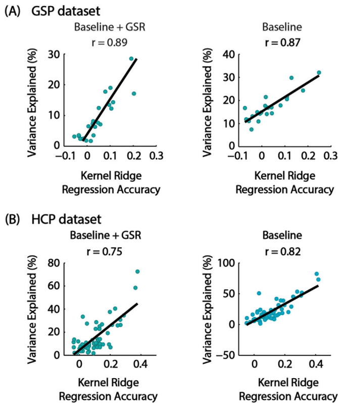
Fig. 7. Consistency across explained behavioral variance and kernel ridge regression accuracies.
