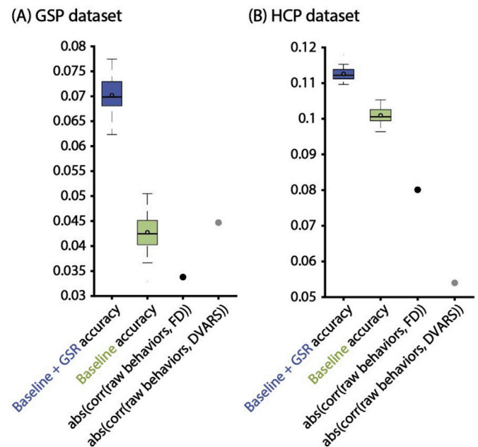
Fig. 12. RSFC-based behavioral prediction accuracies cannot be simply due to motion in the (A) GSP and (B) HCP datasets.
